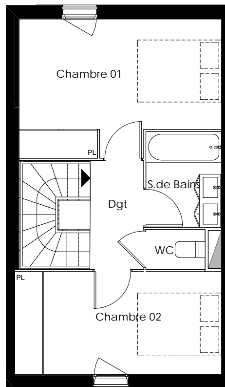
PLAN R+1
