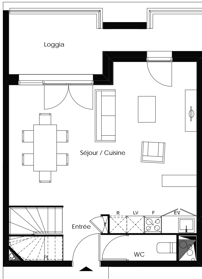
PLAN R+1
